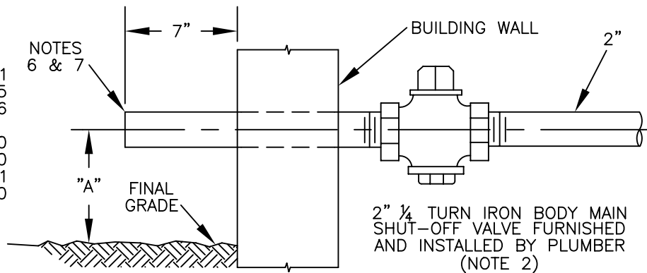
COMMERCIAL AND SMALL INDUSTRIAL CUSTOMER – 2" PIPING
