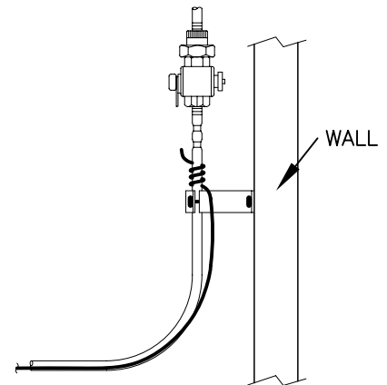
DETAIL "C" TERMINATION AT SERVICE RISER
